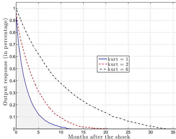
The figure represents an economy with \epsilon = 1 , N(\Delta p_i) = 1.0 and std(\Delta p_i) = 0.10 . The three curves correspond to economies with a steady state kurtosis of the size of price changes equal to 1, 2 and 6, respectively.
